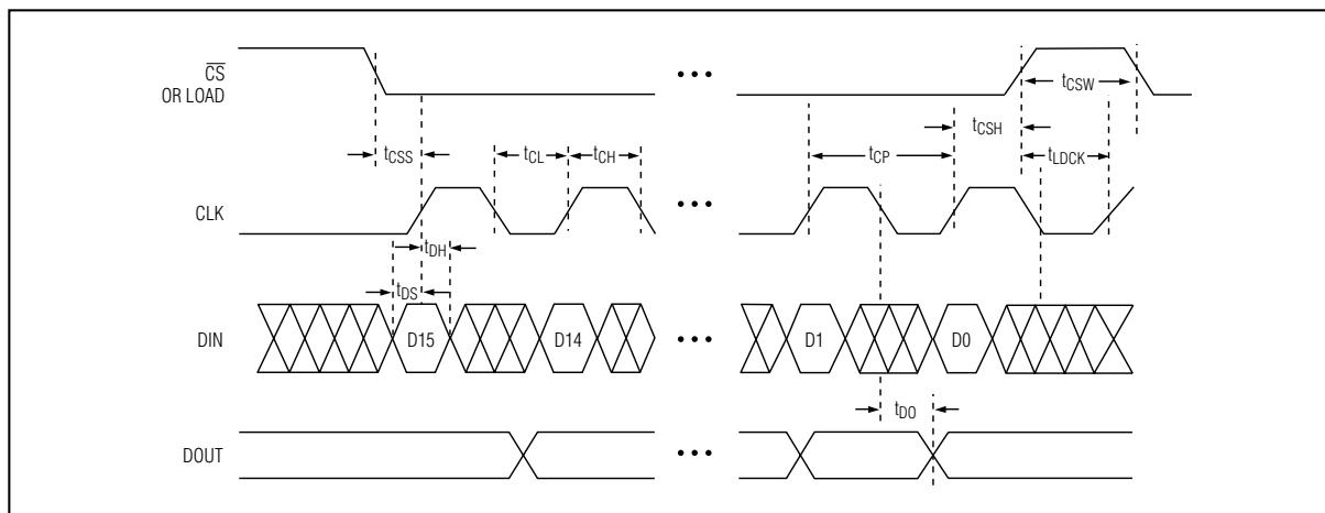
Figure 1. Timing Diagram
